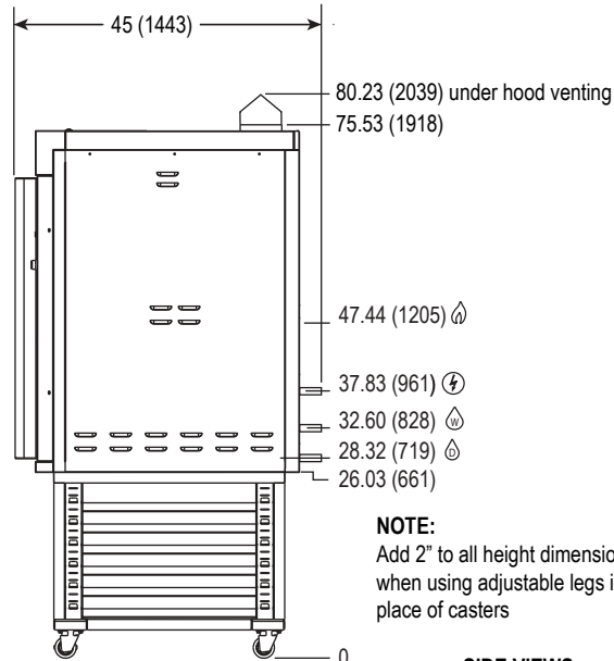
SIDE VIEWS
